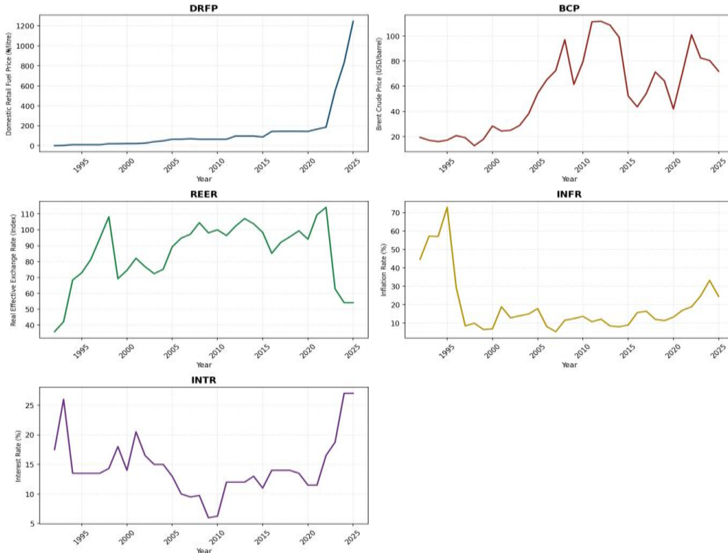
Figure 1. Individual time series plots of study variables (1992-2025). Source: Extract from STATA 17, 2026.
