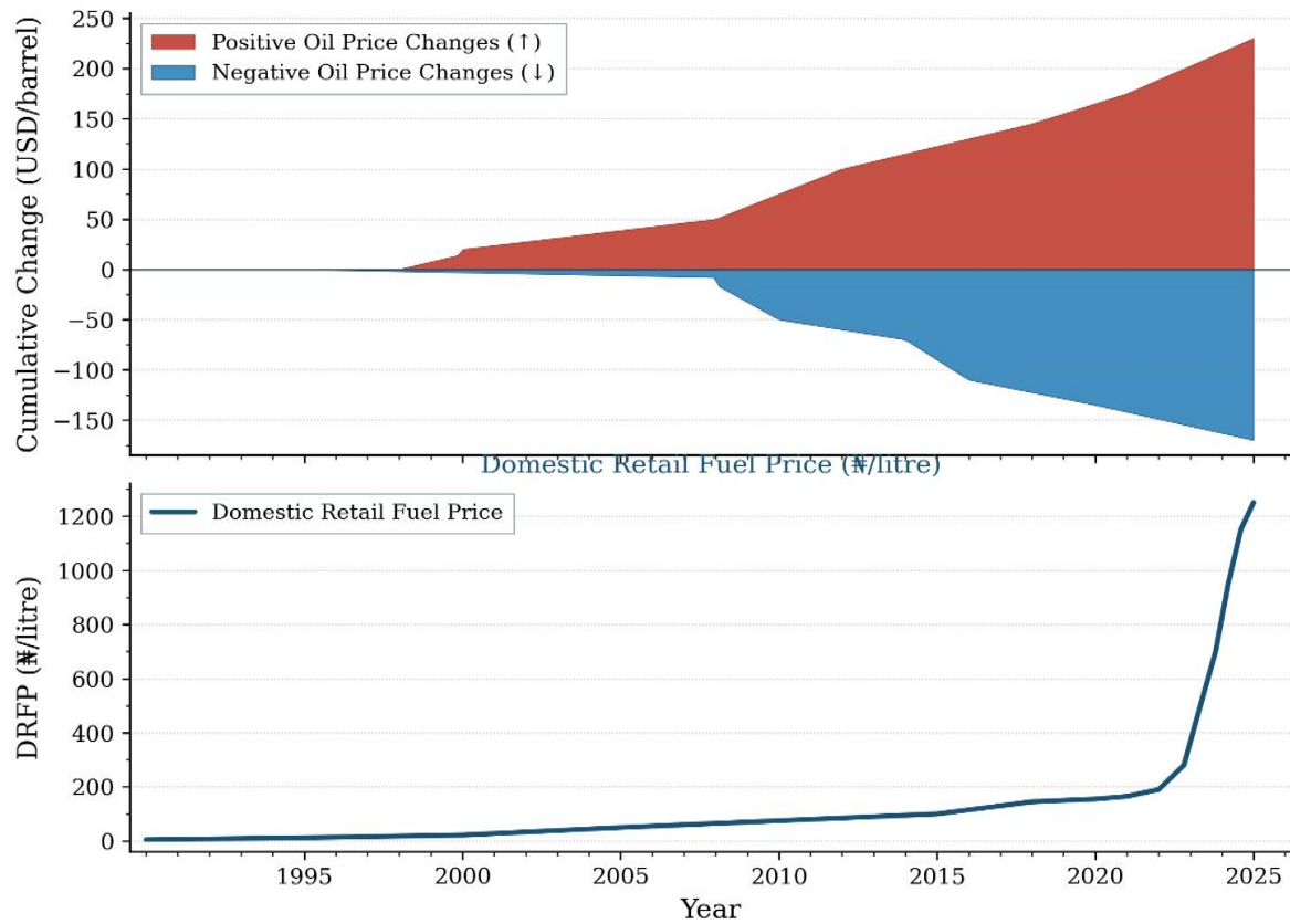
Figure 3. Decomposes changes in BCP into positive and negative partial sum components following the Shin et al., (2014) NARDL framework.
