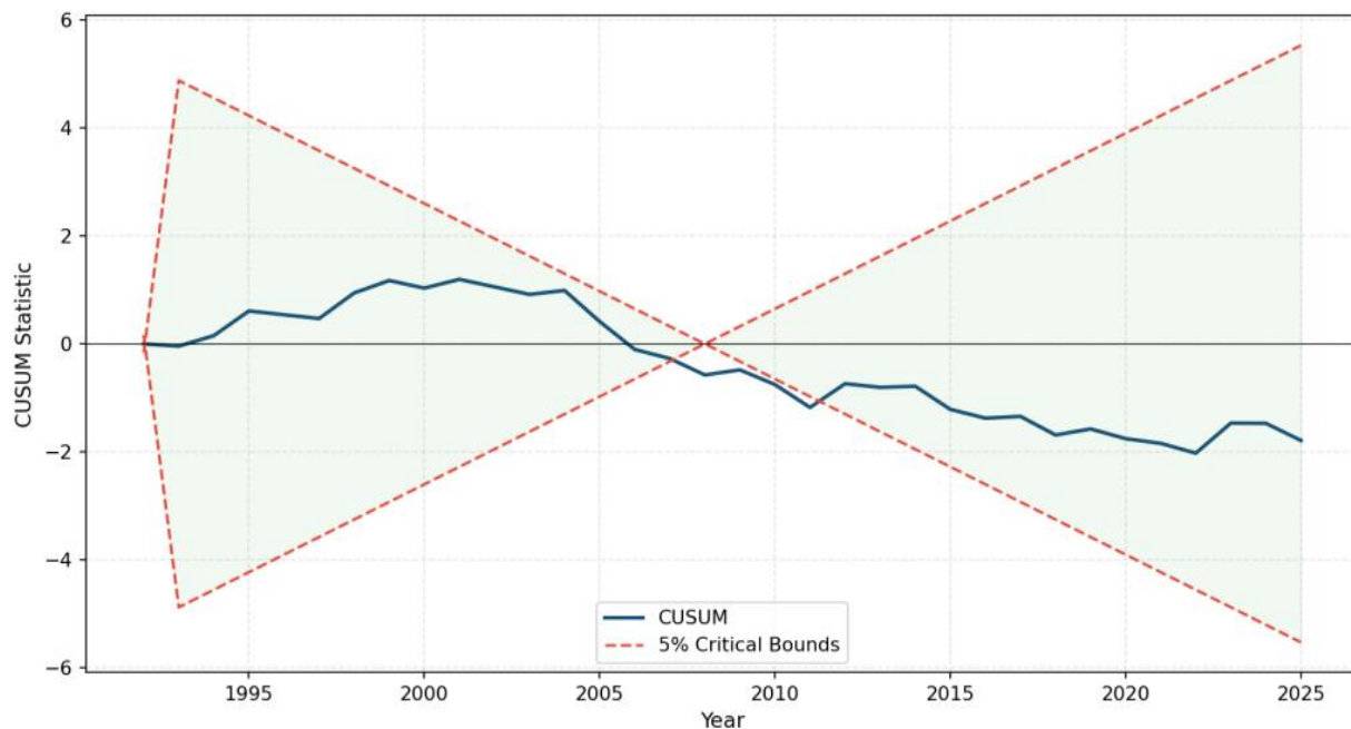
Figure 5. CUSUM test for parameter stability of the Dynamic ARDL model. The CUSUM statistic is plotted against the 5% critical bounds.
