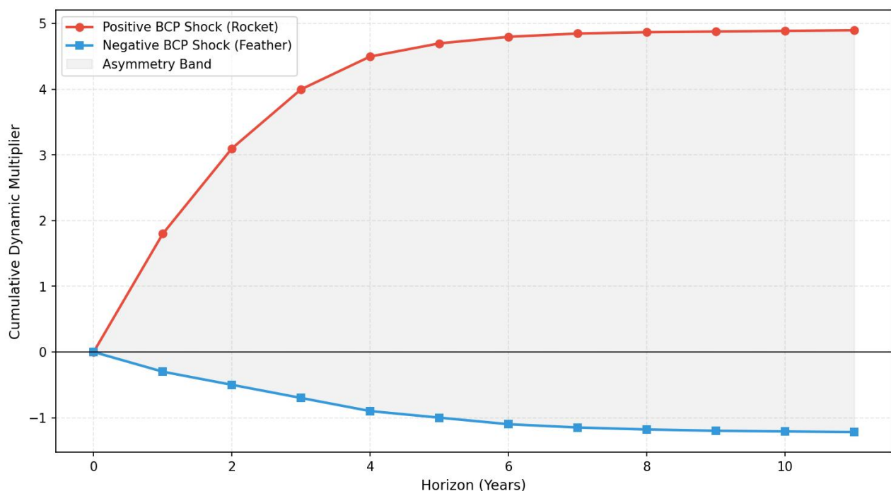
Figure 4. Dynamic multiplier functions—asymmetric response of drfp to bcp shocks.
