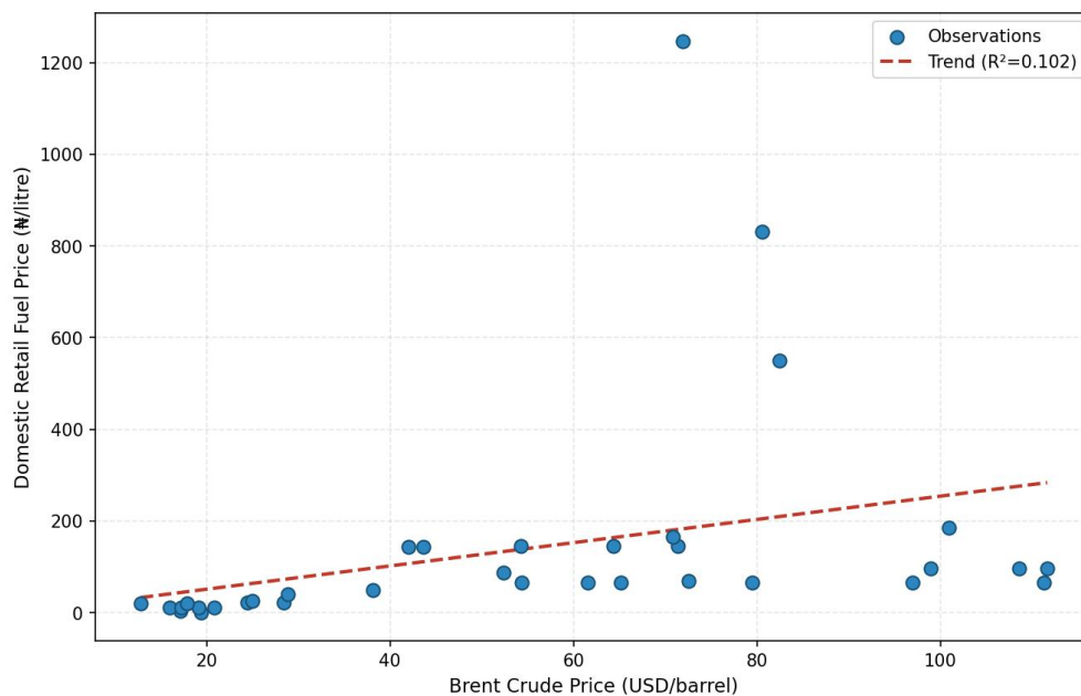
Figure 2. Relationship between BCP and DRFP. Source: Extract from STATA 17, 2026.
